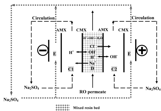
Fig. 2. Mixed bed configuration in the diluate compartment (CMX: cation exchange membrane, AMX: anion exchange membrane, C1: cathodic concentrate, C2: anodic concentrate, D: diluate, E: electrode rinsing).
